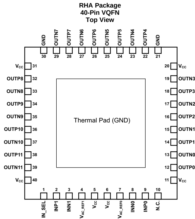
Pin Functions
