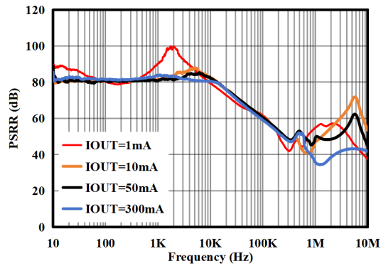
Figure 9. PSRR
