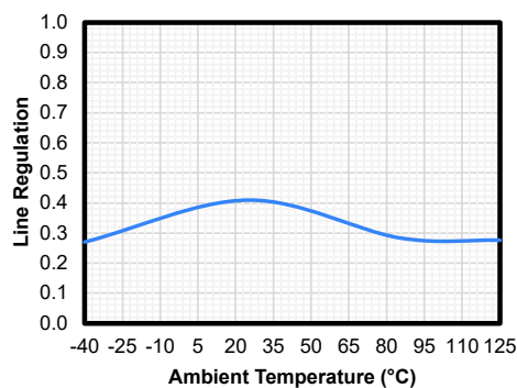
Figure 3. Line Regulation
