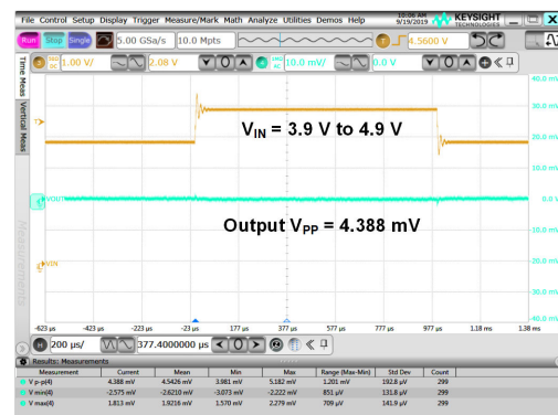
Figure 10. Noise
