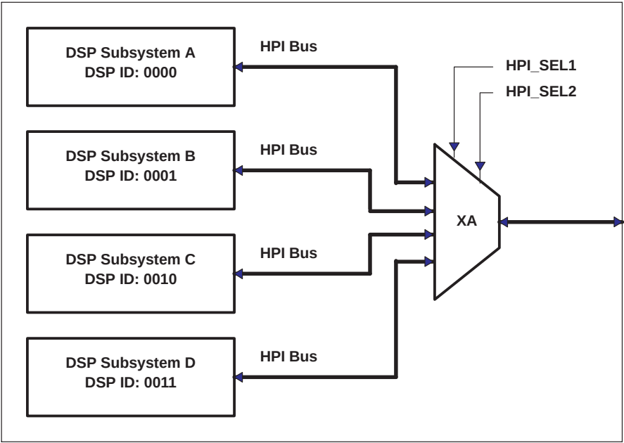
Figure 3–14. XA Multiplexer for HPI Access
