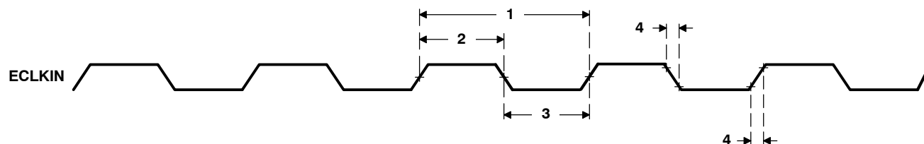
Figure 24. ECLKIN Timings
