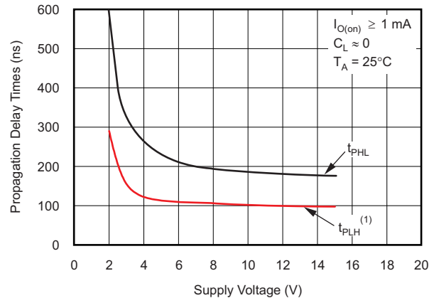
Figure 2. Propagation Delay Times to Discharge Output From Trigger and Threshold Shorted Together vs Supply Voltage
