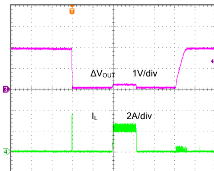
Short Circuit Protection ( V_{IN}=5.0V , V_{OUT}=1.8V , I_{LOAD}=0A -Short, SY8003A)
