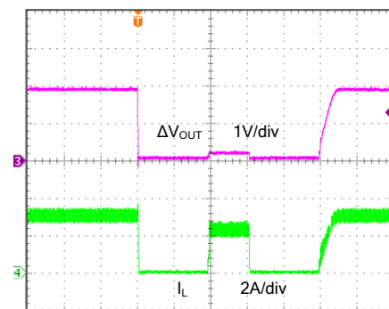
Short Circuit Protection ( V_{IN}=5.0V , V_{OUT}=1.8V , I_{LOAD}=3.0A -Short, SY8003A)
