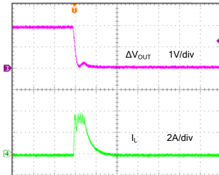
Short Circuit Protection ( V_{IN}=5.0V , V_{OUT}=1.8V , I_{LOAD}=0A -Short SY8003)
