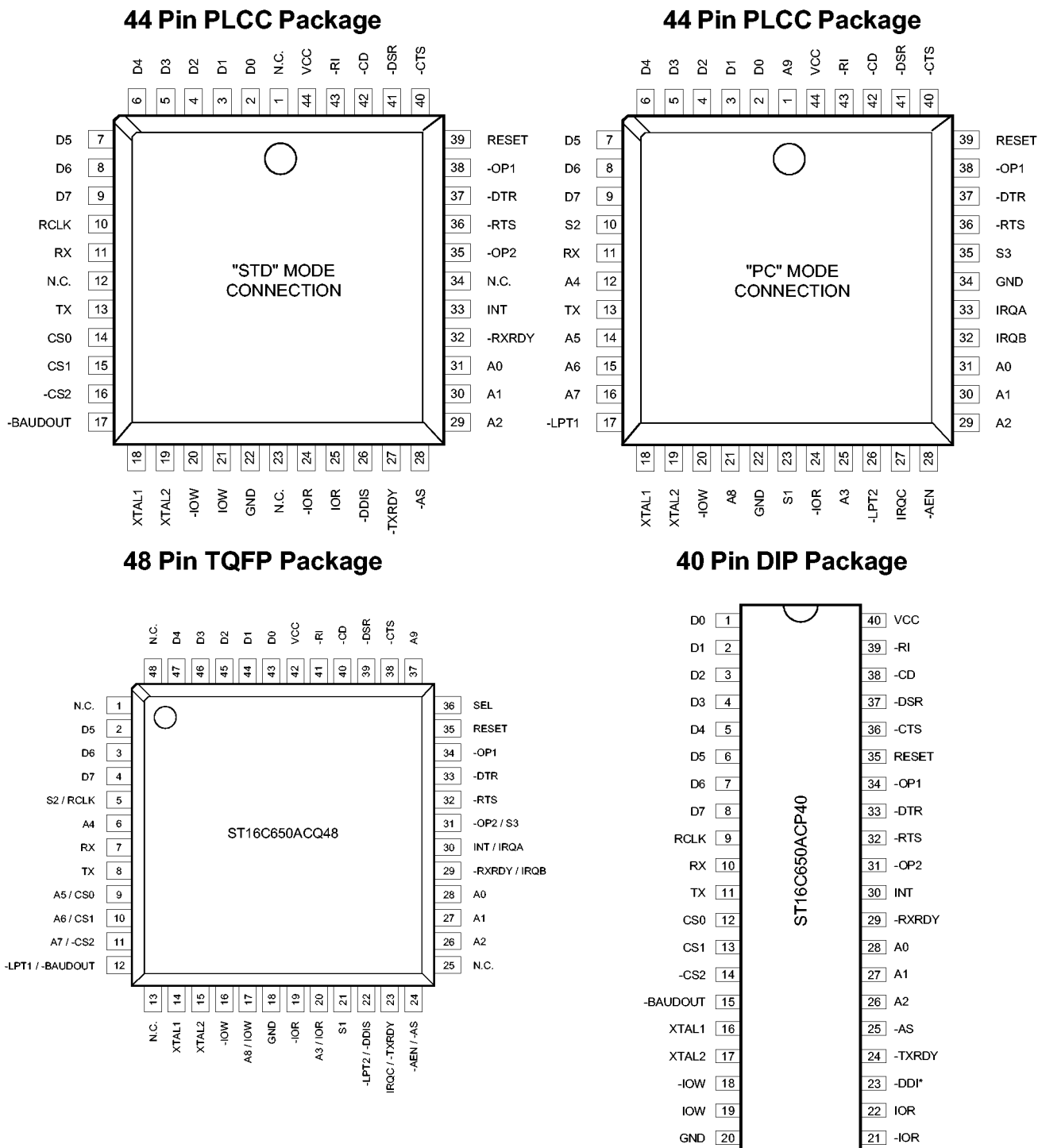
Figure 1, PACKAGE DESCRIPTION, 16C650A
