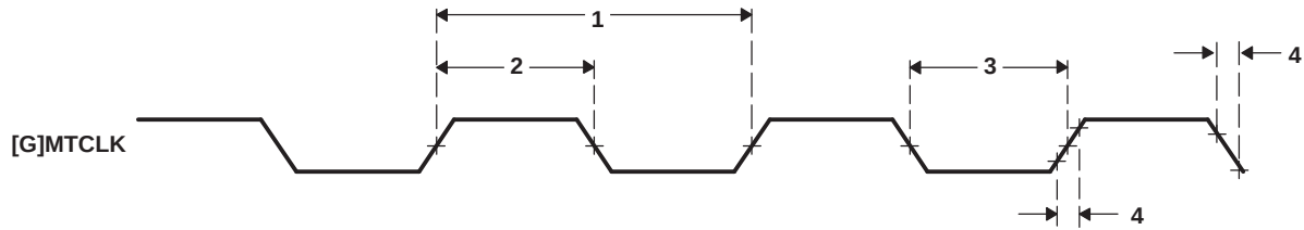
Figure 7-49. [G]MTCLK Timing
