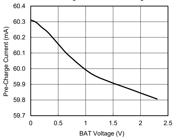
Pre-Charge Current vs. BAT Voltage
