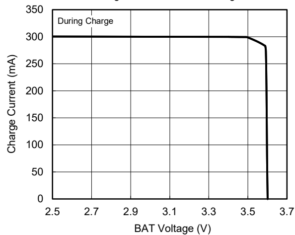
Charge Current vs. BAT Voltage
