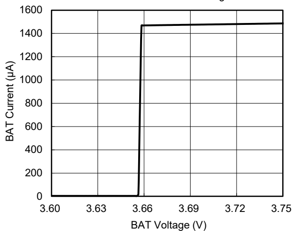
BAT Current vs. BAT Voltage
