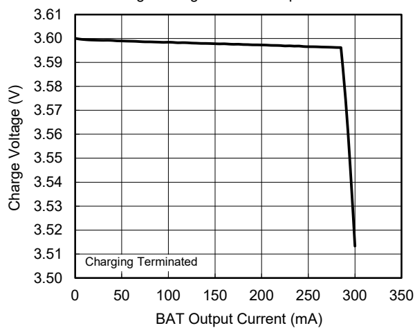
Charge Voltage vs. BAT Output Current
