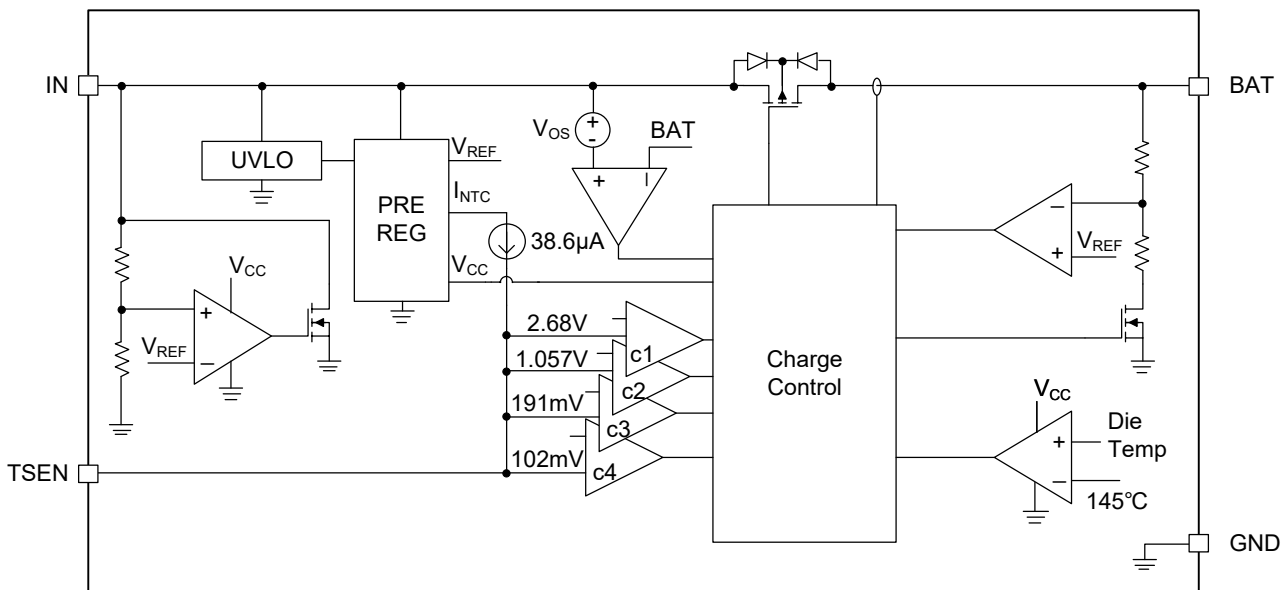
Figure 4. Block Diagram
