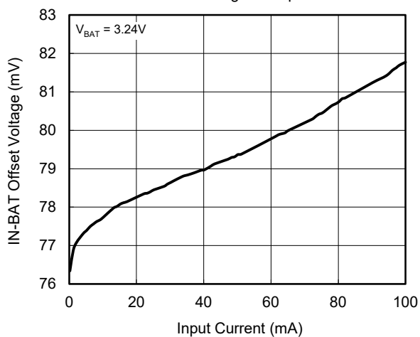
IN-BAT Offset Voltage vs. Input Current
