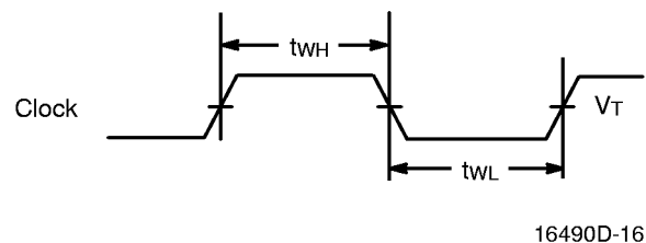
Clock Width
