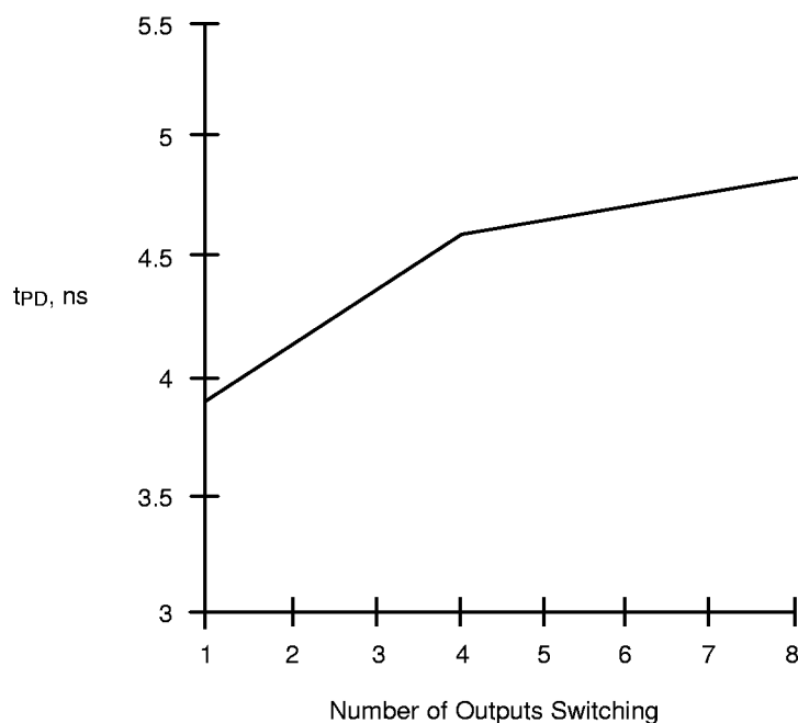
t_{PD} vs. Number of Outputs Switching V_{CC} = 4.75 V, T_A = 75^\circ\text{C} (Note 1)
