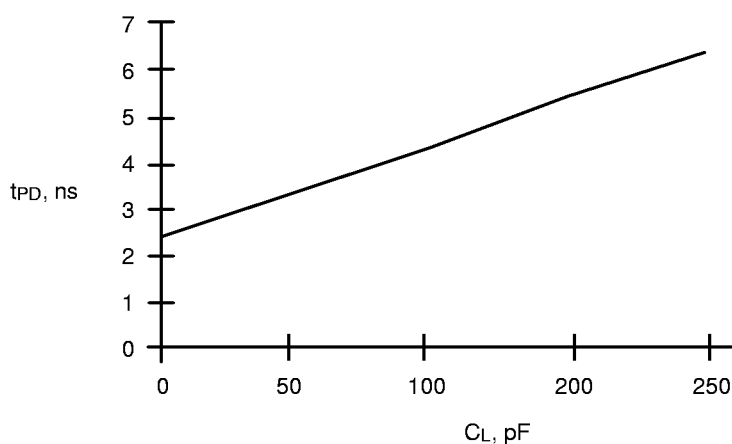
t_{PD} vs. Load Capacitance V_{CC} = 5.0 V, T_A = 25^\circ\text{C}
