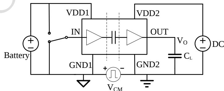
Figure 2.11 Common-Mode Transient Immunity Test Circuit
