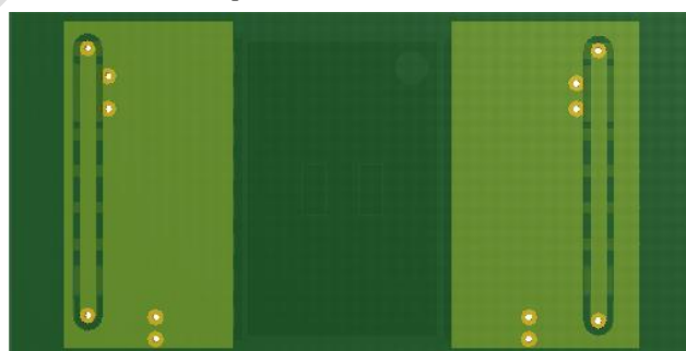
Figure 5.2 Recommended PCB Layout — Bottom Layer
