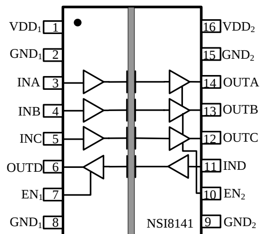
Figure 6.6 NSi8141W Package
