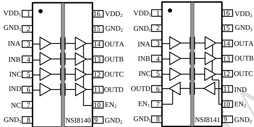
Figure 6.1 NSi8140N Package
