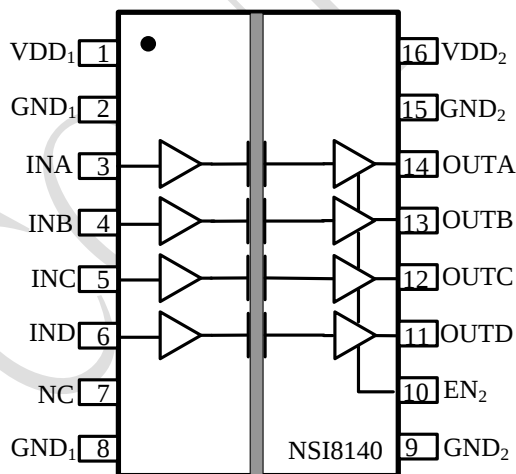
Figure 6.5 NSi8140W Package
