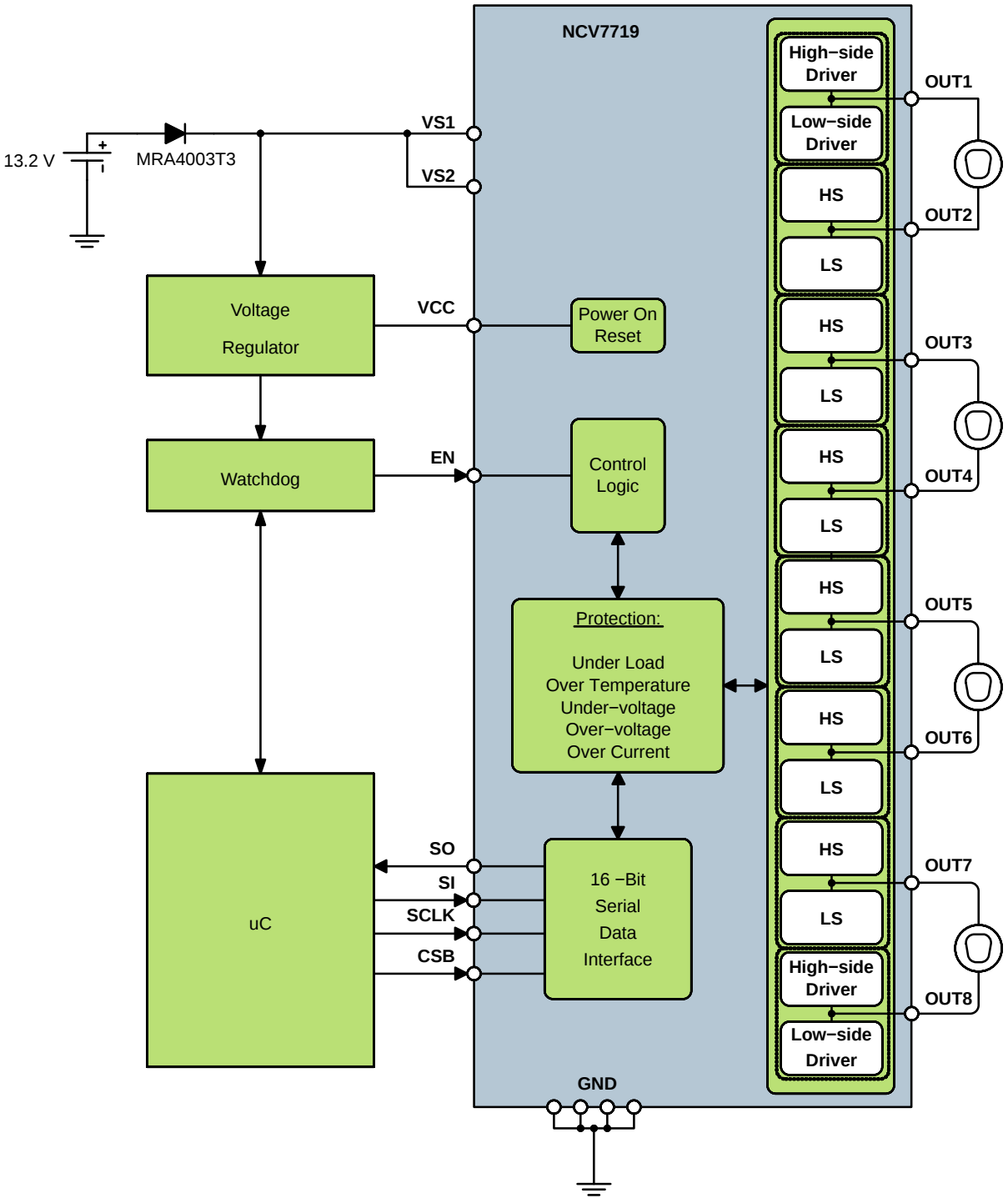
Figure 1. Typical Application
