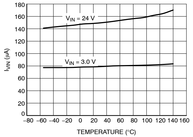
Figure 12. V_{IN} Controller Current vs. Temperature ( EN = V_{CC} )
