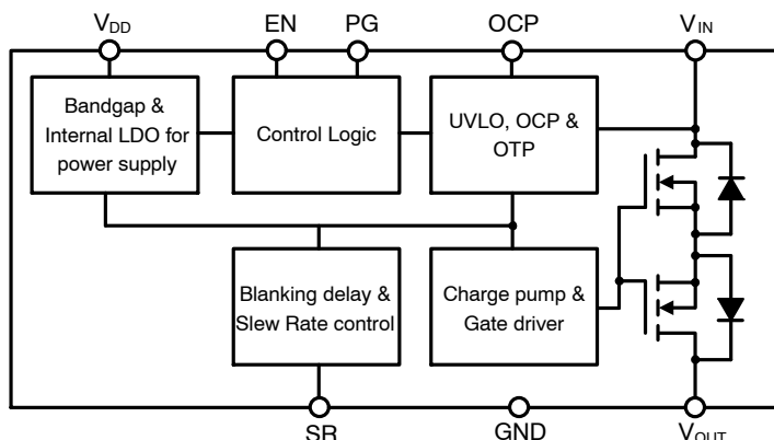
Figure 1. Block Diagram
