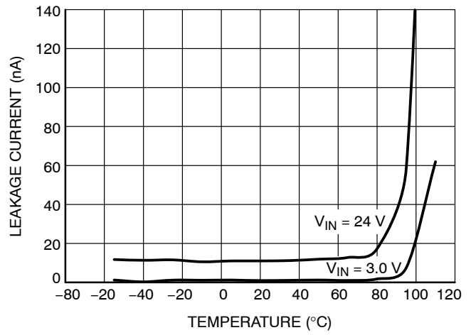
Figure 10. Input to Output Leakage vs. Temperature
