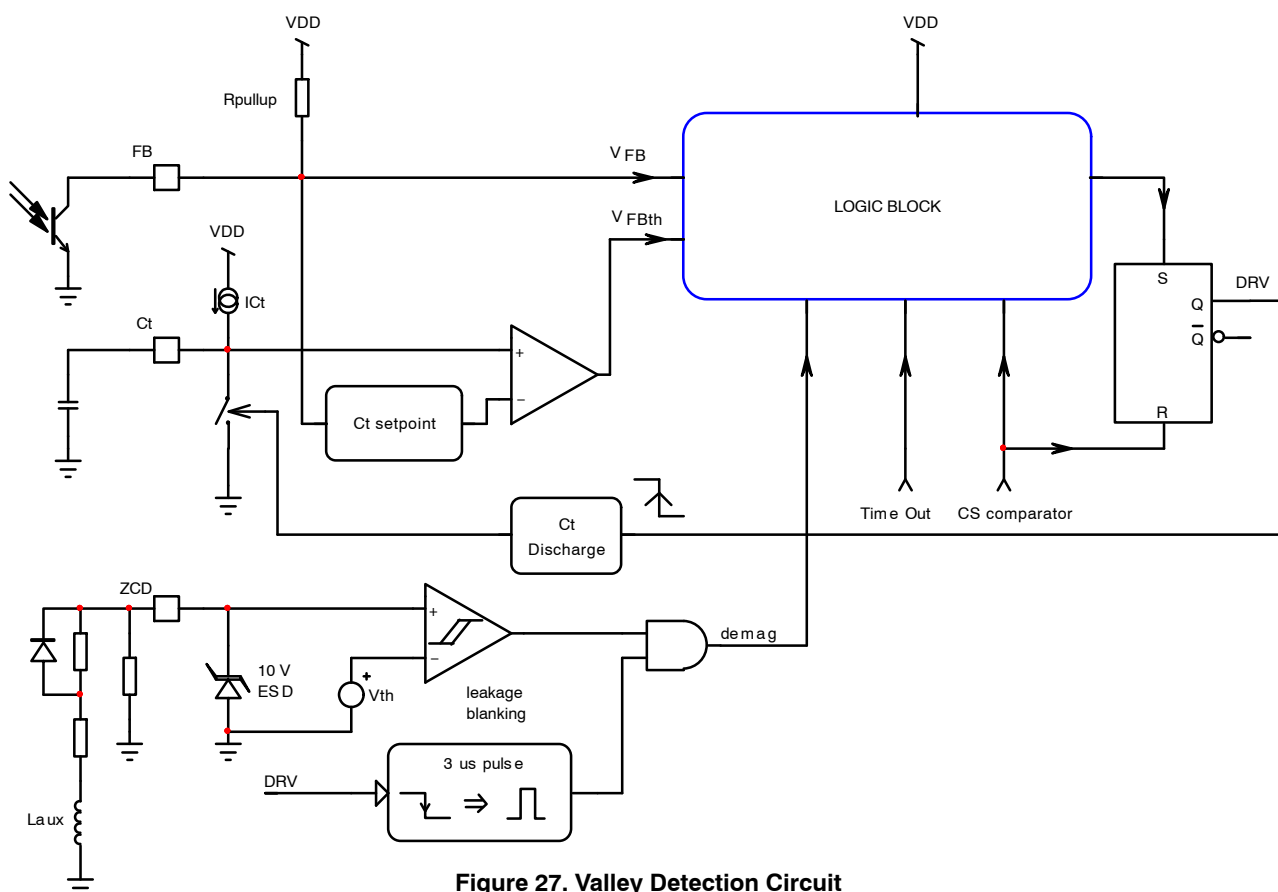
Figure 27. Valley Detection Circuit
