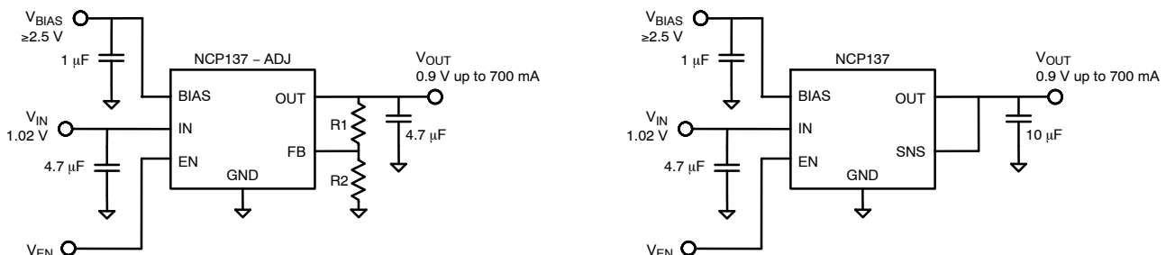
Figure 1. Typical Application Schematics
