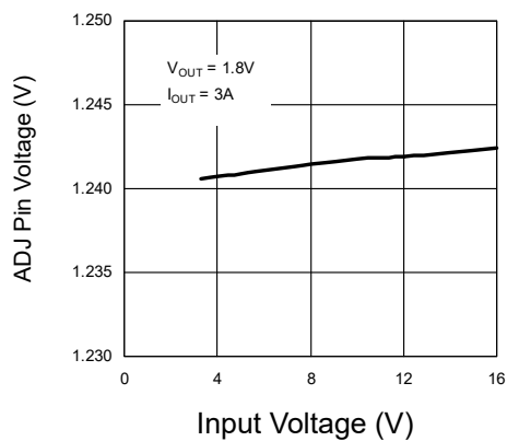
Figure 3: Adjust Pin Voltage vs. Input Voltage
