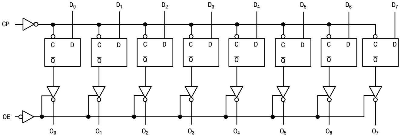
Figure 3. Logic Diagram
