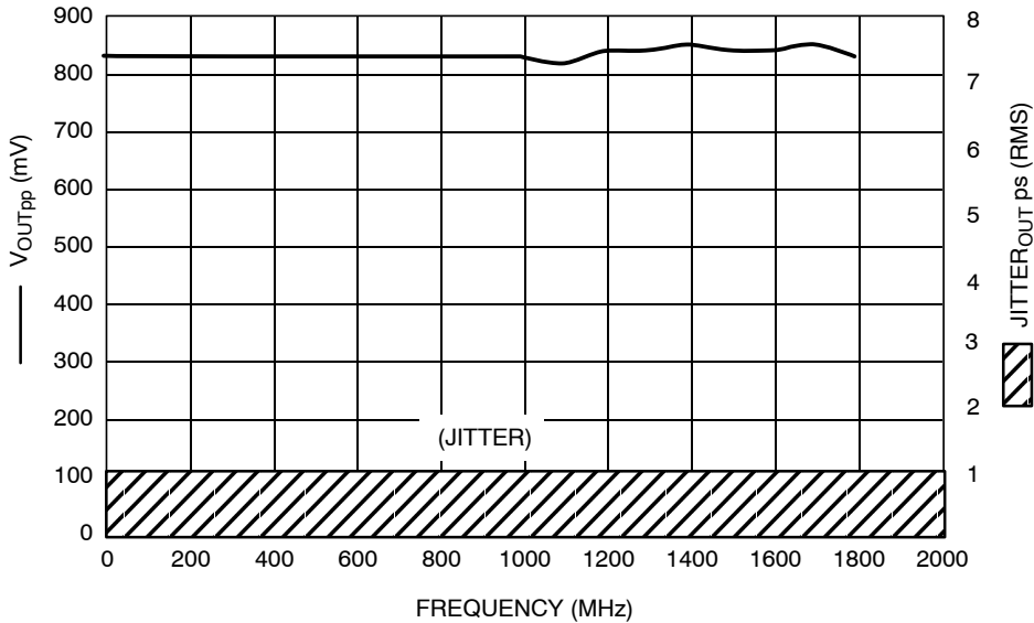
Figure 5. \div 2 , F_{max}/Jitter
