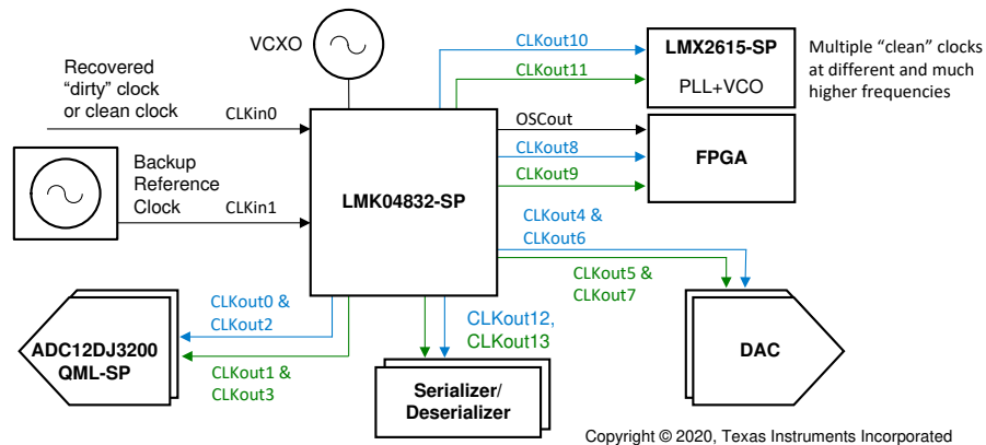
Figure 9-6. Typical Application
