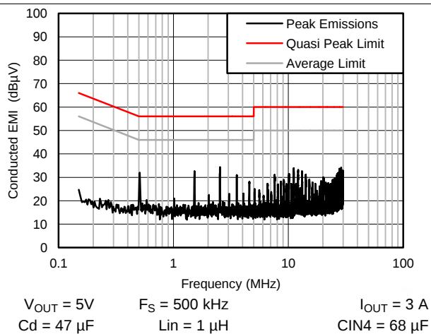
Figure 34. LM43603PWPEVM Conducted EMI Curve
