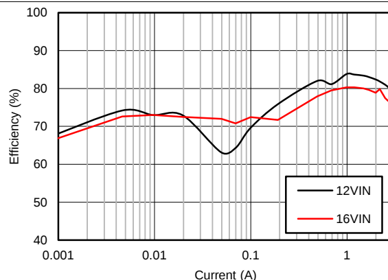
Figure 86. Efficiency
