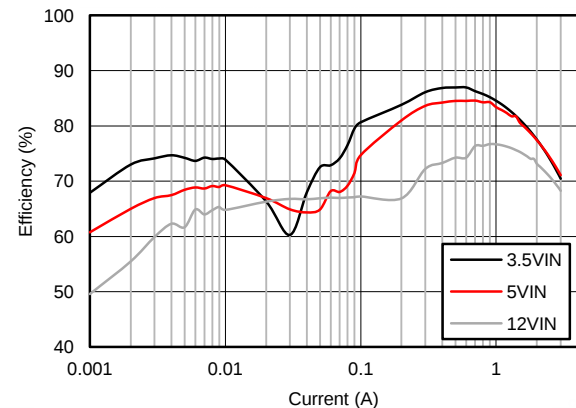
Figure 50. Efficiency
