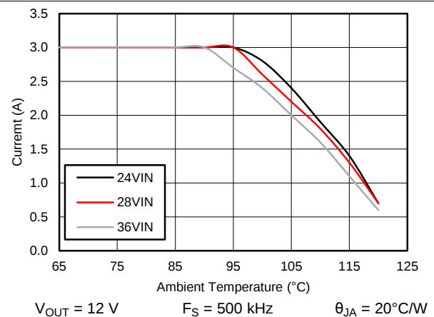
Figure 96. Derating Curve
