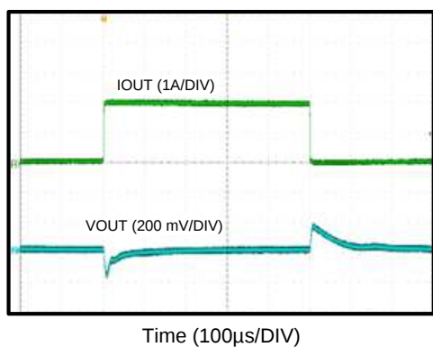
Figure 65. Load Transient 0.1A to 2A
