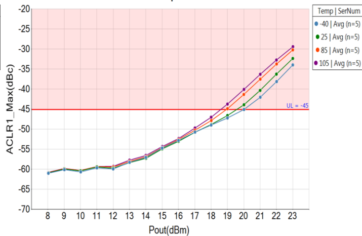
GRF5110 ACLR1 vs Pout at Modulation = LTE_20MHz_100RB and Freq = 2000 MHz
