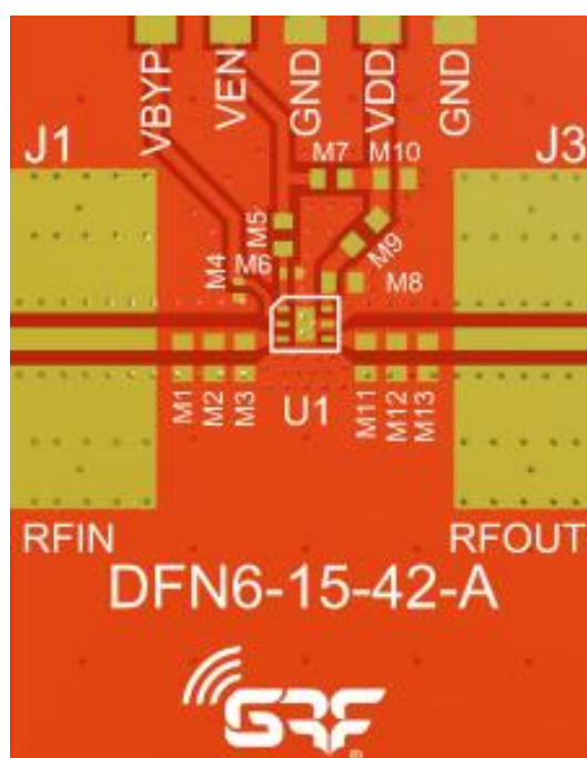
GRF2541 Evaluation Board Assembly Diagram
