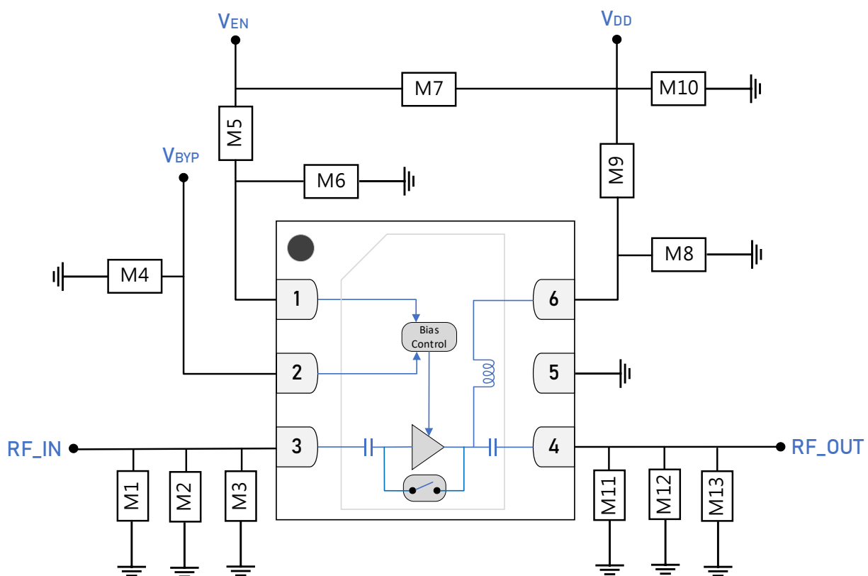
GRF2541 Standard Evaluation Board Schematic
