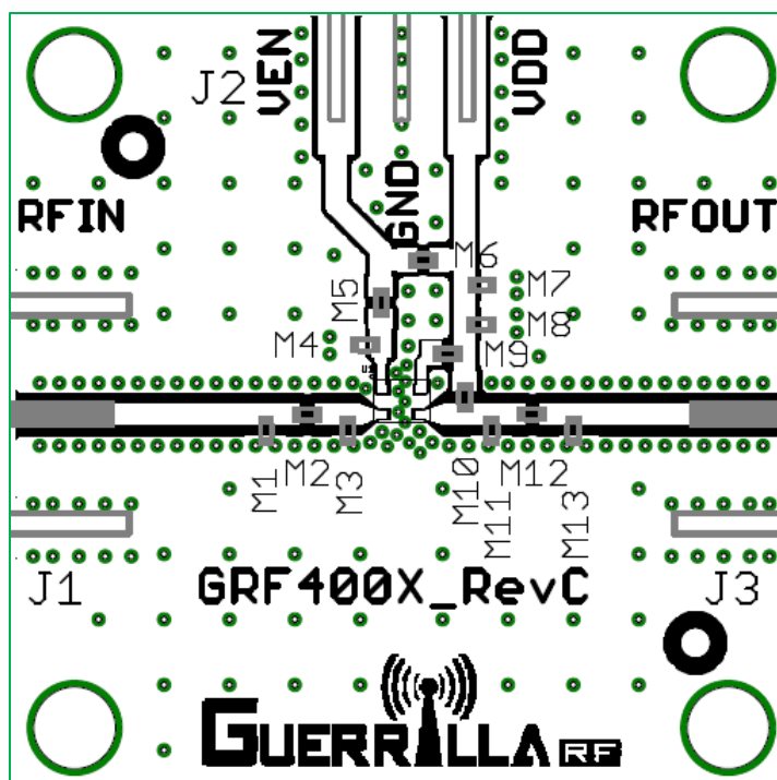
GRF2505 Evaluation Board Assembly Diagram
