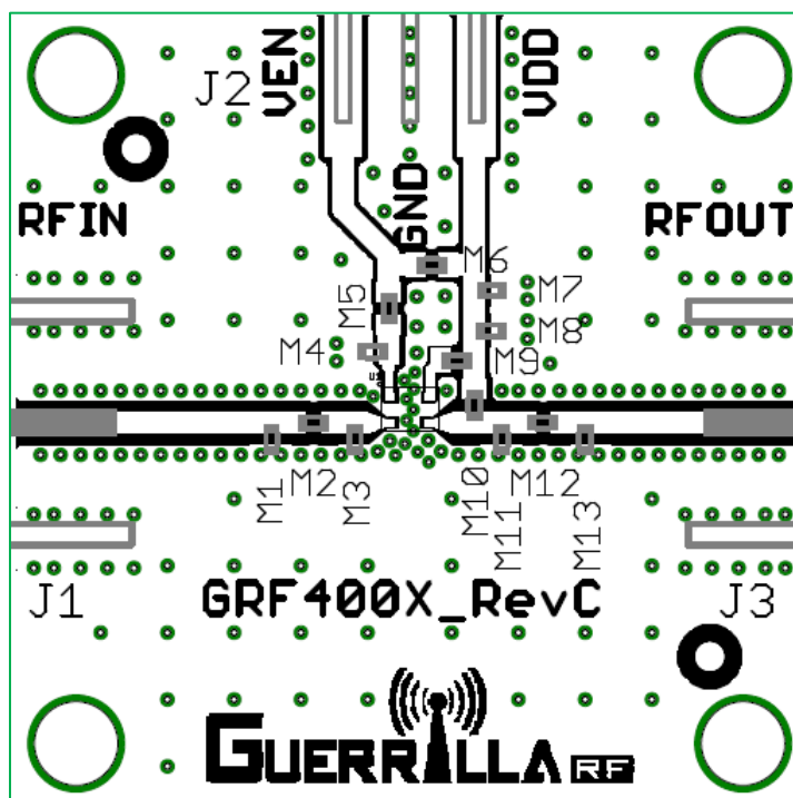
GRF2373 Evaluation Board Assembly Diagram
