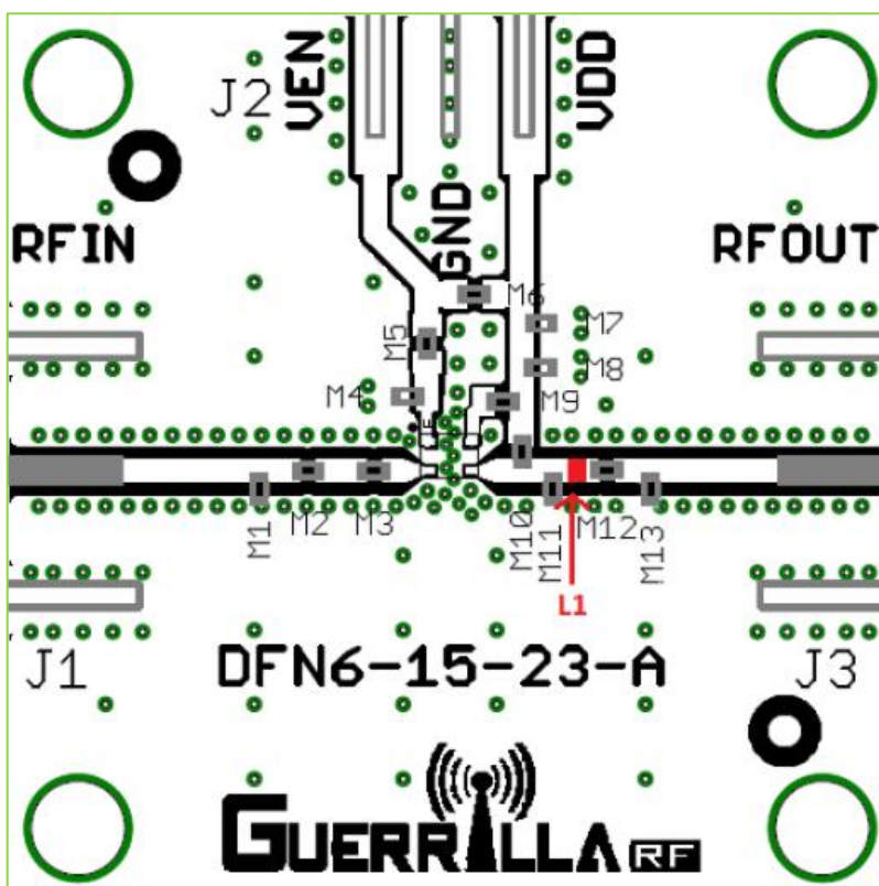
GRF2100 Evaluation Board Assembly Diagram
