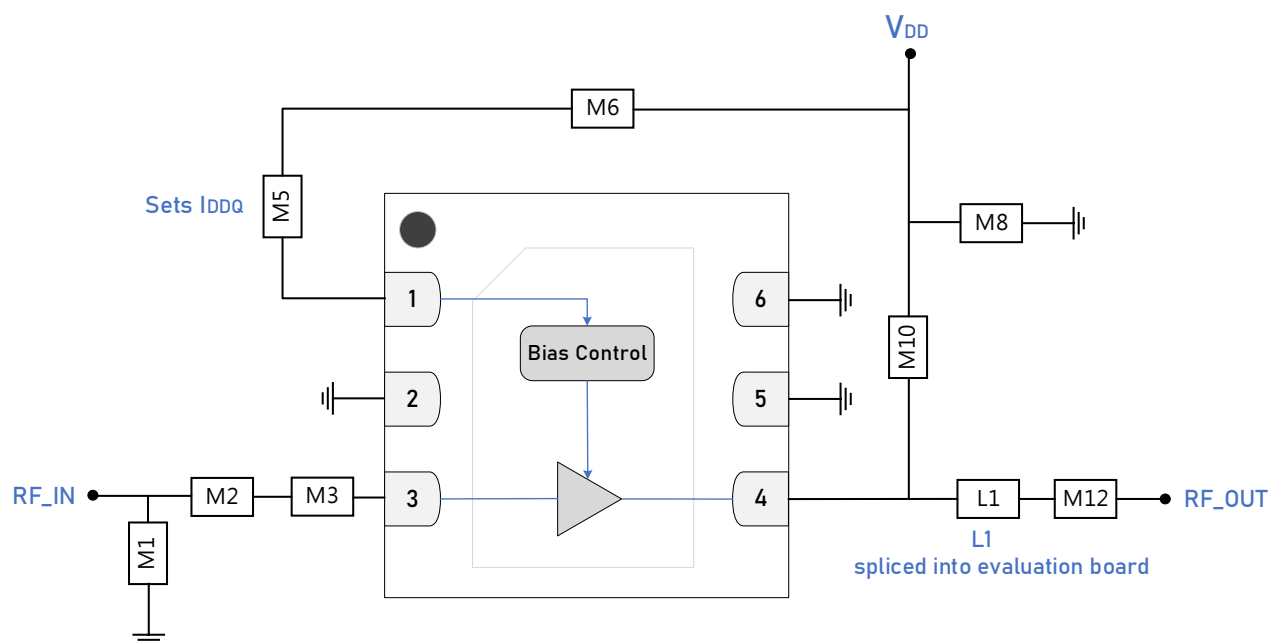
GRF2100 Standard Evaluation Board Schematic
