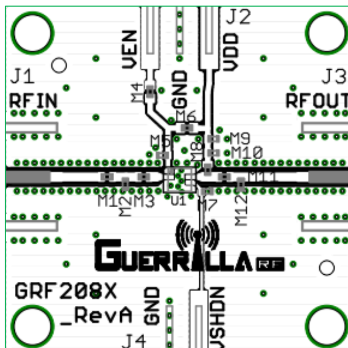
GRF2080 Evaluation Board Assembly Diagram
