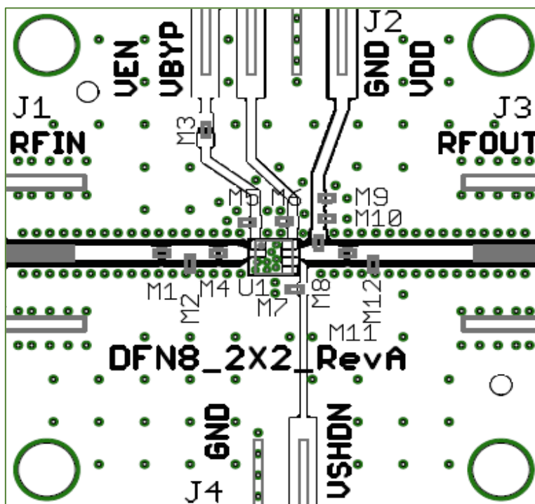
GRF2073 Evaluation Board Assembly Diagram
