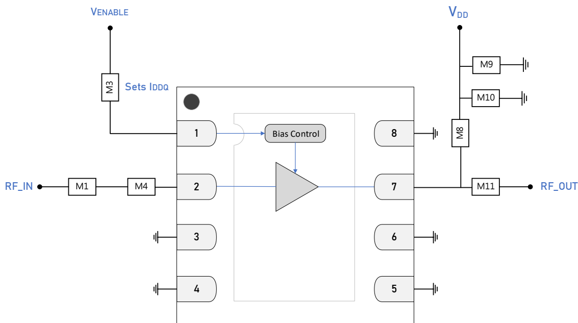
GRF2073 Standard Evaluation Board Schematic
