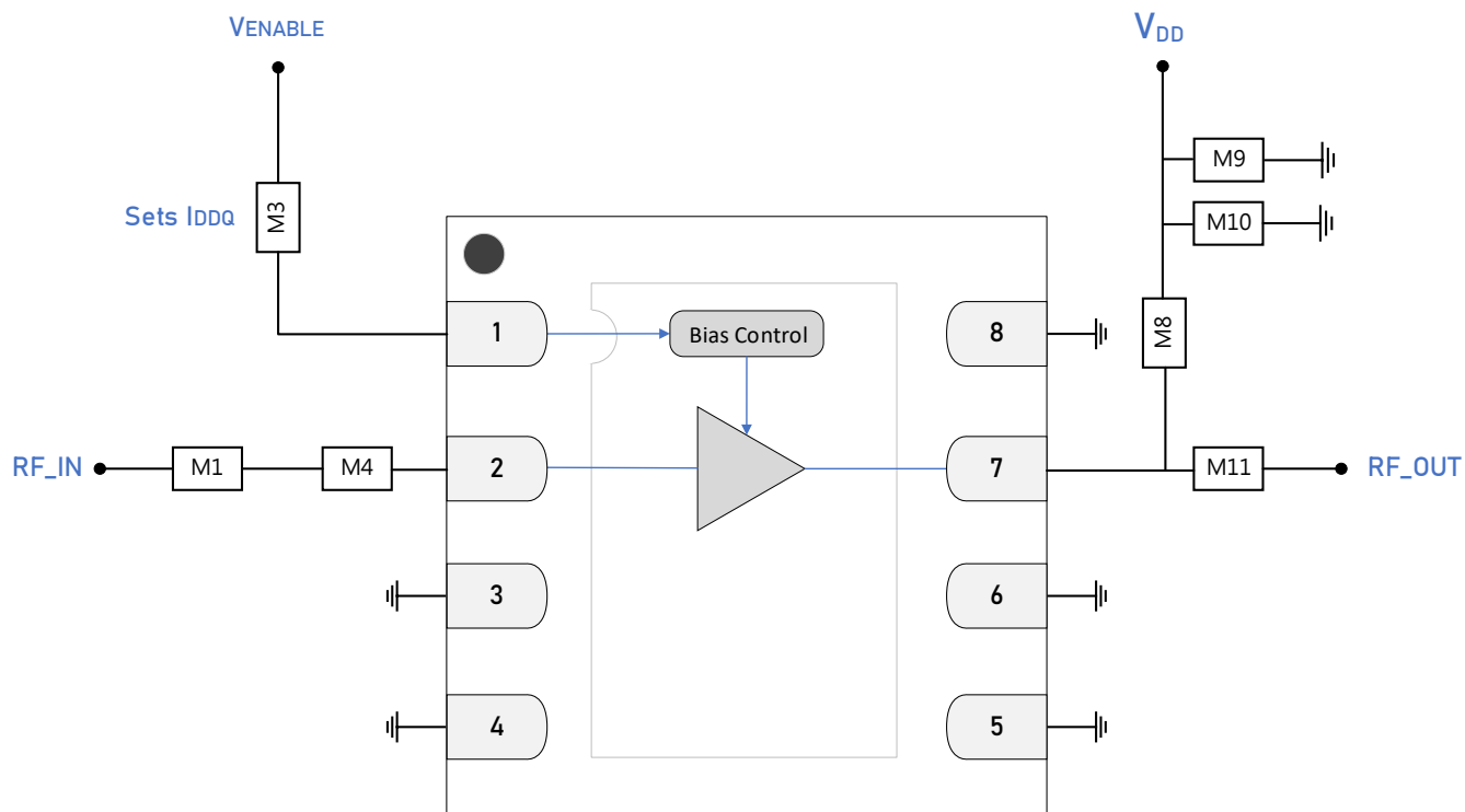
GRF2071 Standard Evaluation Board Schematic
