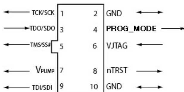
Figure 19 · FlashPro5 10-Pin Connector
