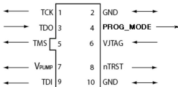
Figure 20 · FlashPro4 10-Pin Connector
