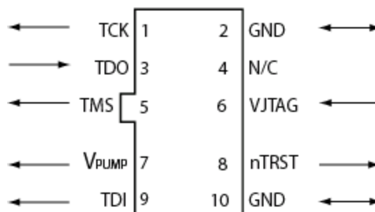
Figure 21 · FlashPro3 10-Pin Connector
