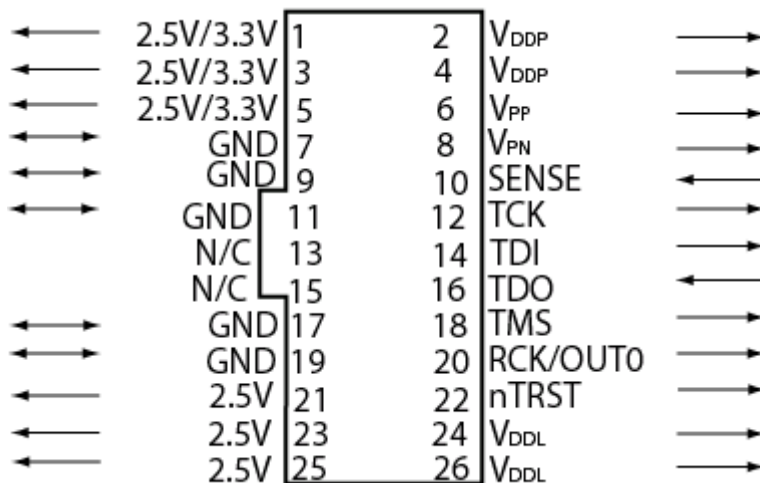
Figure 22 · 26-pin connections for FlashPro
