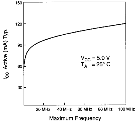
Figure 23. EP22V10 I_{CC} vs. Frequency
