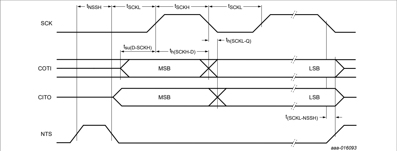
Figure 9. Connection to host with SPI
