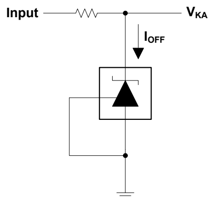
Figure 3. Test Circuit for I_{OFF}
