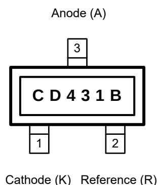
CD431B SOT-23 Package
