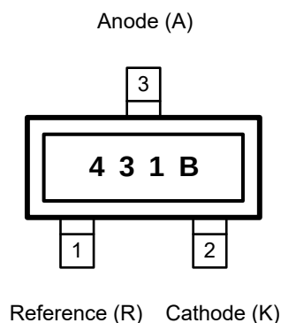
CJ431B SOT-23 Package
