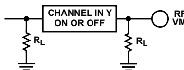
Figure 6-15. Crosstalk Between Duals or Triplets ()
