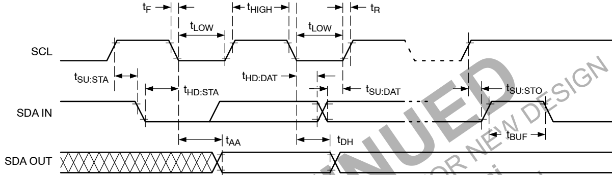
Figure 2. Bus Timing
