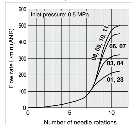
AS2201FSG□-02, AS2211FSG□-02
