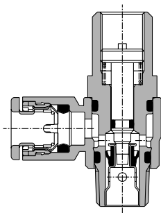
Meter-in type
