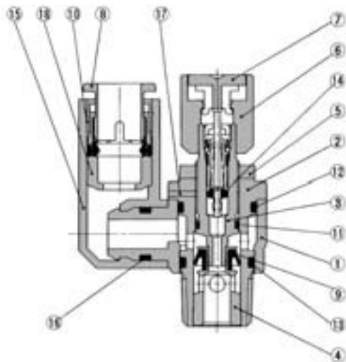
Meter-in type
