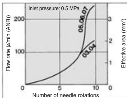
AS2001FG
