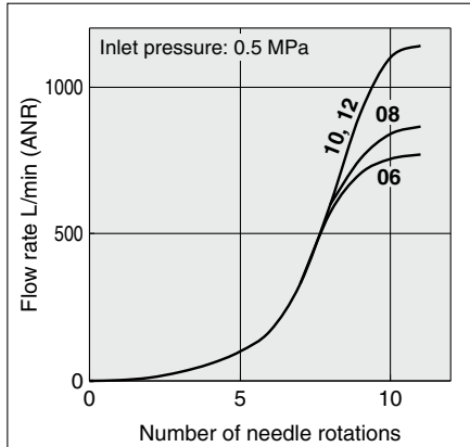
AS3301F, AS3311F
