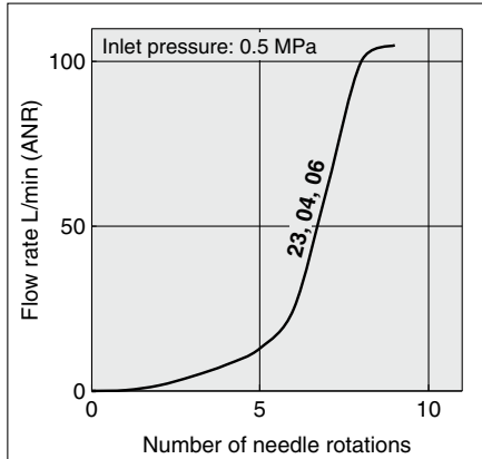
AS1301F-M5□, AS1311F-M5□
