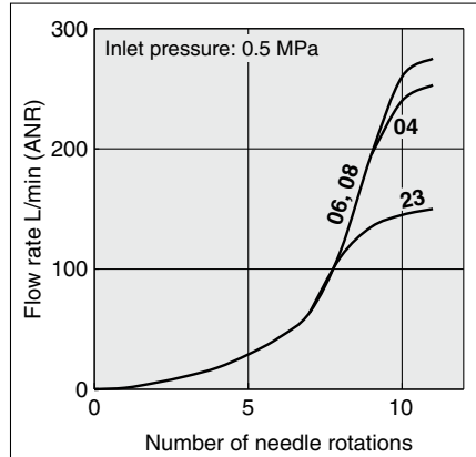
AS2301F-01, AS2311F-01
