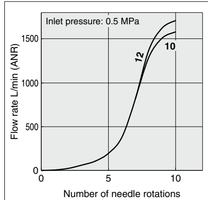
AS4301F, AS4311F
