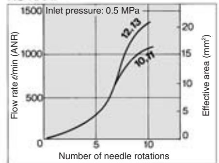
AS4001F
