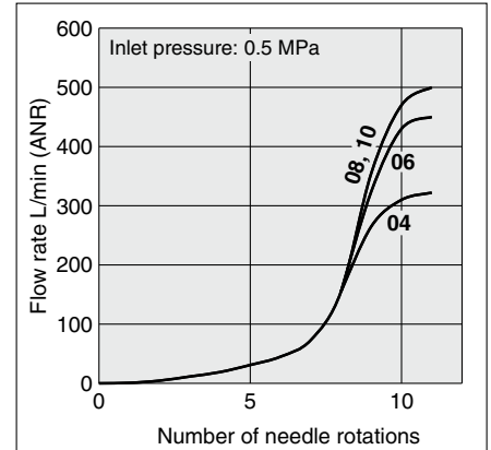
AS2301F-02, AS2311F-02
