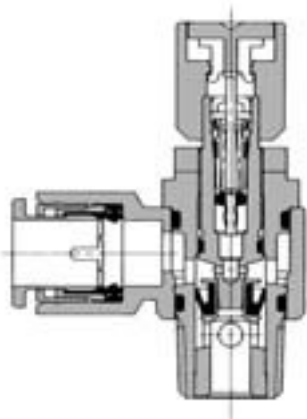
Meter-in type
