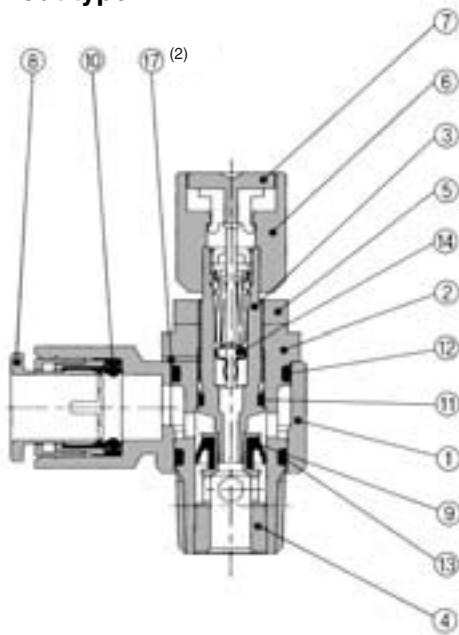
Meter-in type
