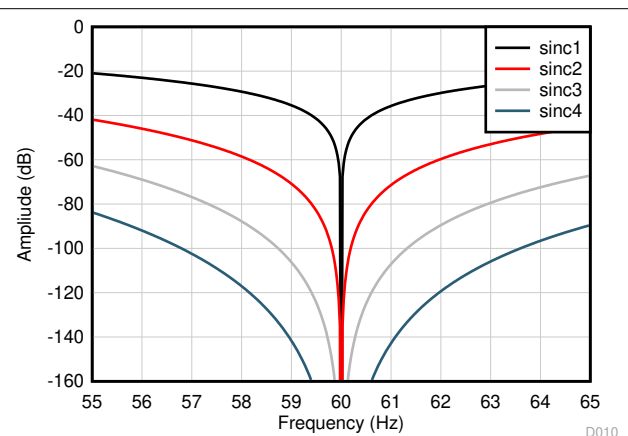
Figure 9-21. Sinc Frequency Response Zoom (60 SPS)
