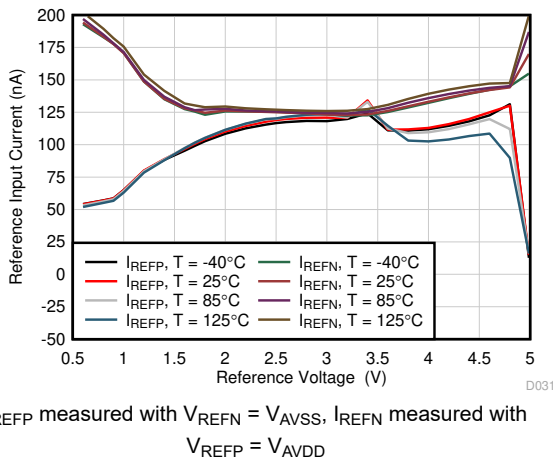
Figure 7-34. ADC1 Reference Input Current
