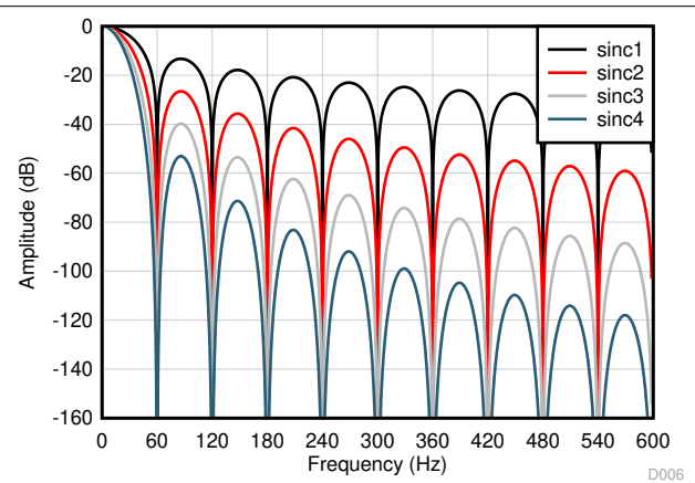
Figure 9-19. Sinc Frequency Response (60 SPS)
