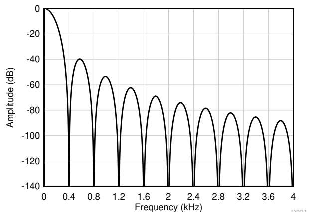
Figure 9-35. ADC2 400 SPS Frequency Response
