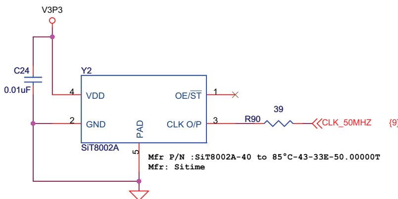
Figure 29 • Clock Oscillator Schematic
