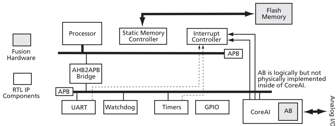
Figure 27 • Embedded Processor System Using CoreAI
