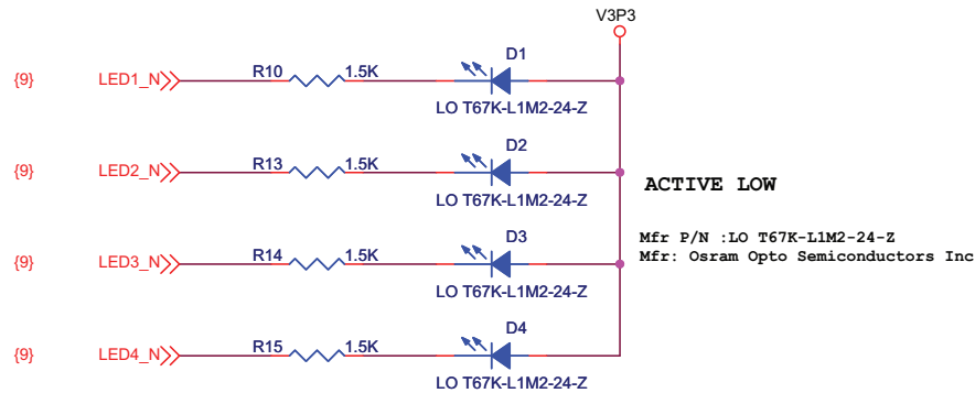
Figure 35 • LEDs Schematic
