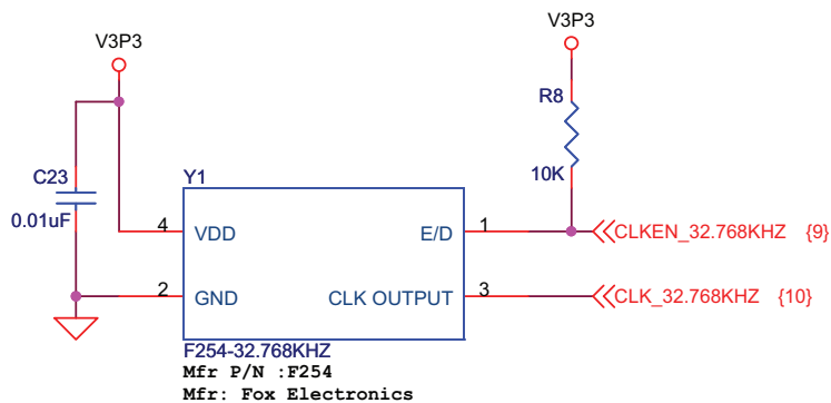
Figure 31 • Off-Chip Crystal Oscillator Schematic
