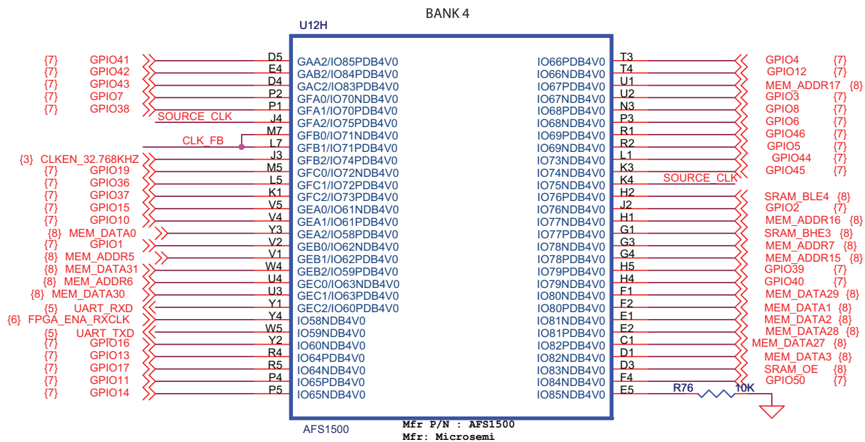
Figure 11 • I/O Pins Schematic for Bank 4
