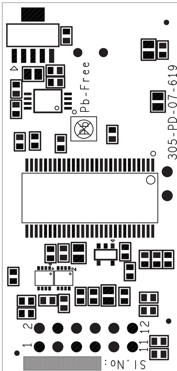
Figure 48 • Low-Cost Programming Stick (LCPS) Stackup (Bottom Silkscreen)
