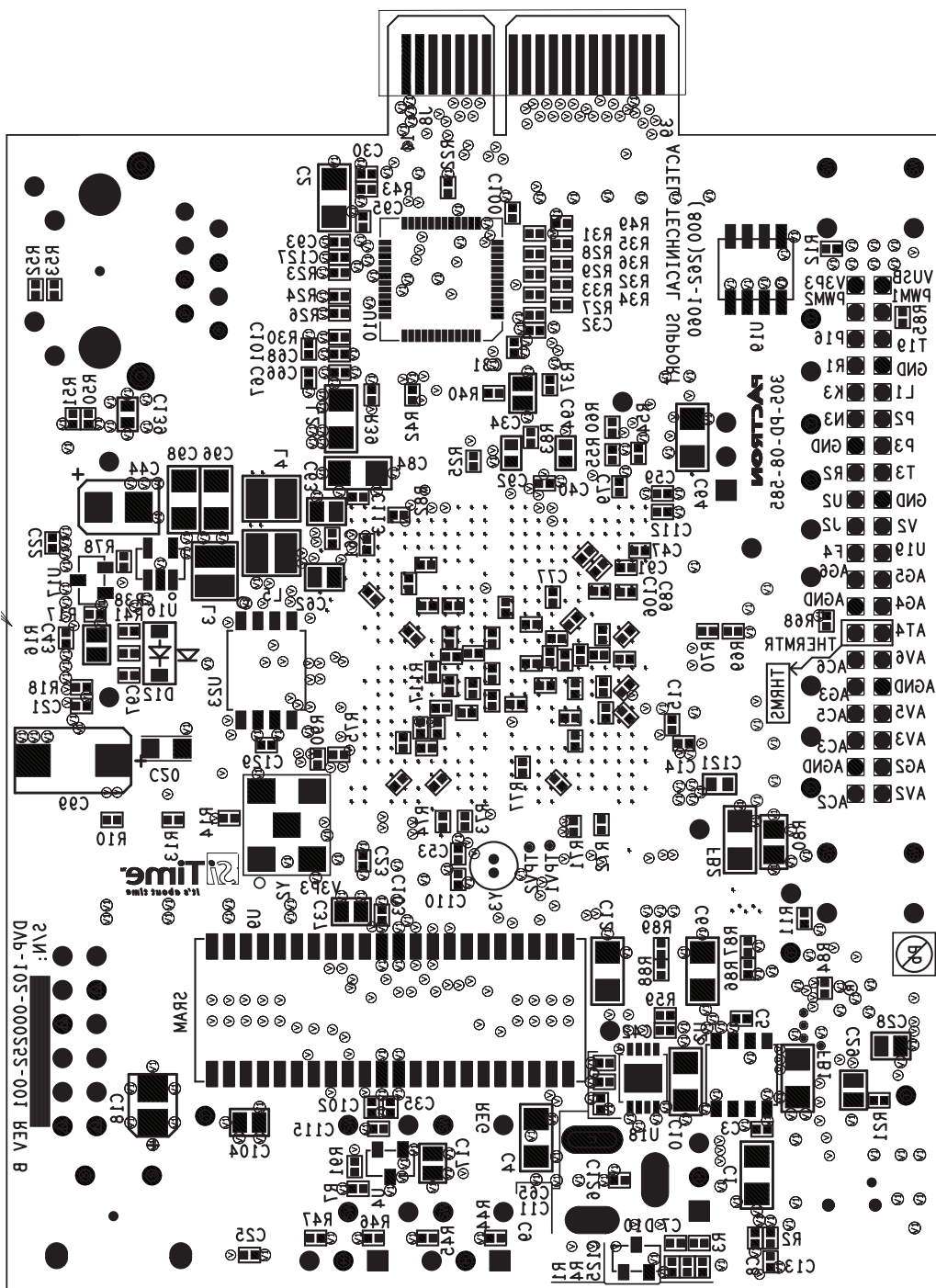
Figure 4 • Bottom Silkscreen
