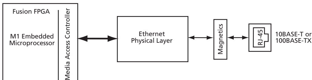
Figure 40 • Typical Application
