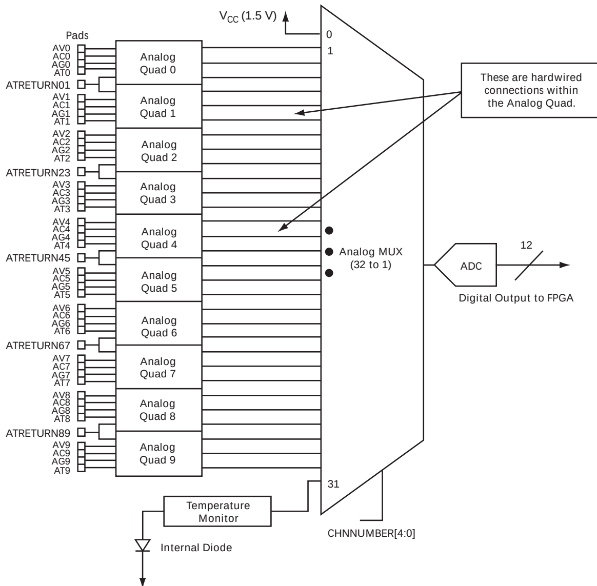
Figure 12 • Analog Block ADC and MUX Architecture
