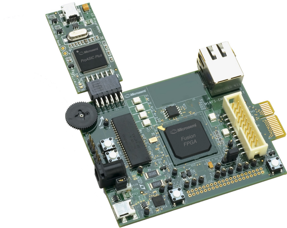
Figure 1 • Fusion Embedded Development Kit Evaluation Board with LCPS Attached
