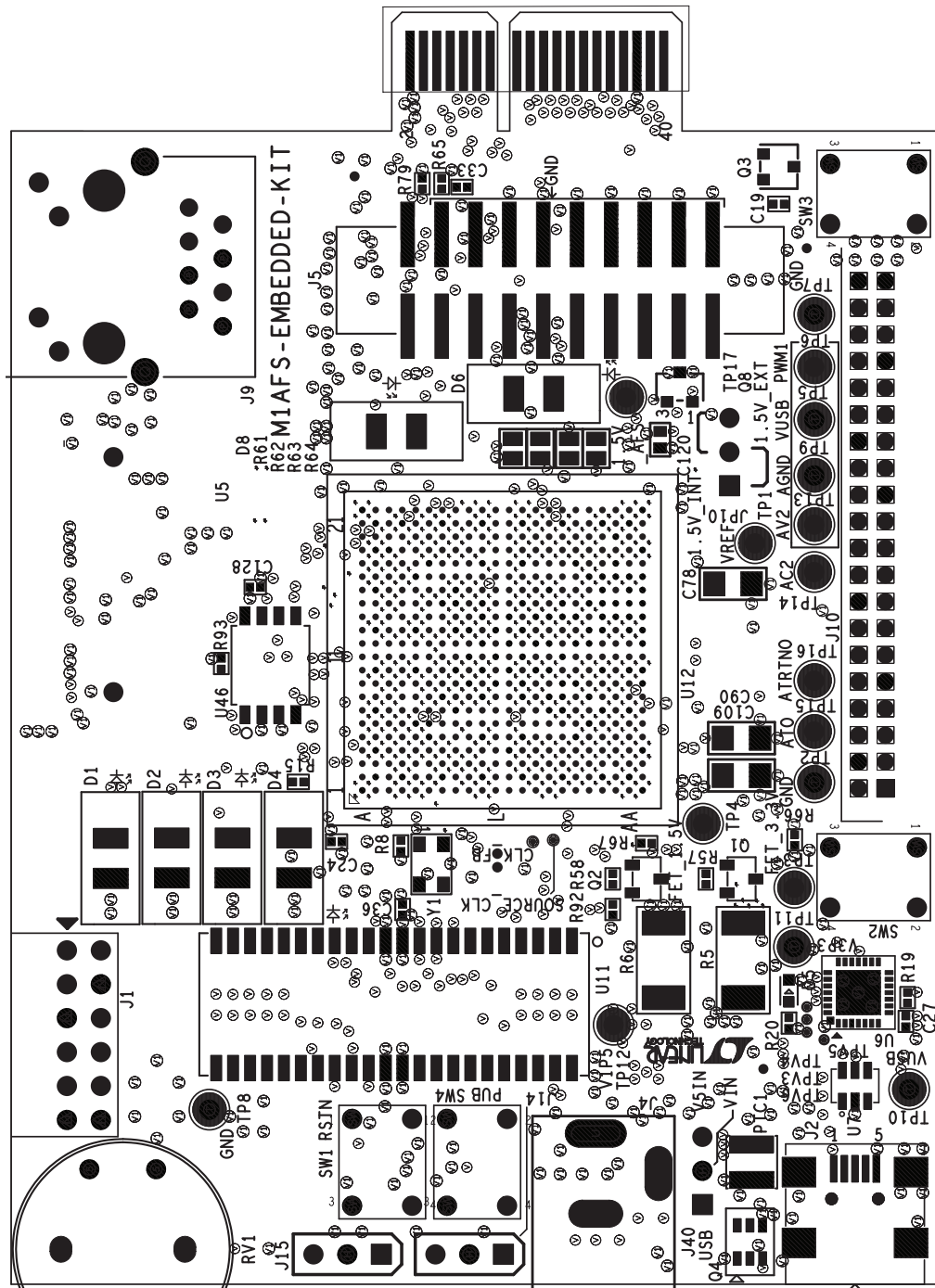
Figure 3 • Top Silkscreen
