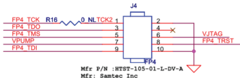
Figure 44 • FlashPro4 Header
