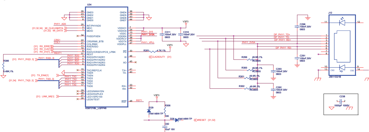
Figure 39 • EtherCat Port1
