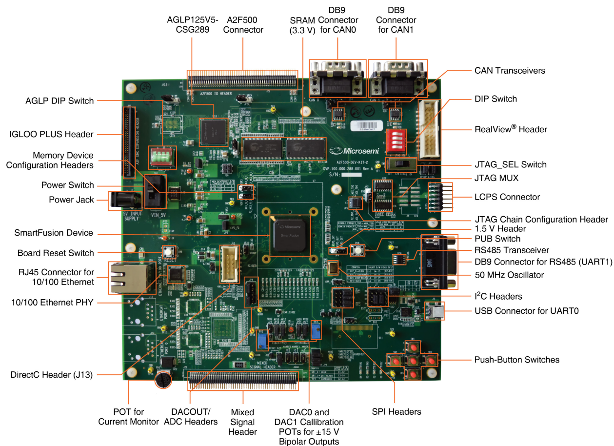
Figure 1 • A2F500-DEV-KIT-2
