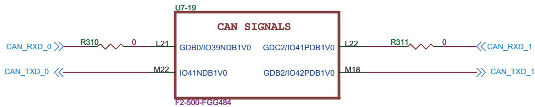
Figure 36 • CAN Interface
