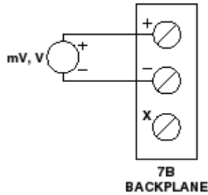
Figure 3 7B30 Input Field Connections
