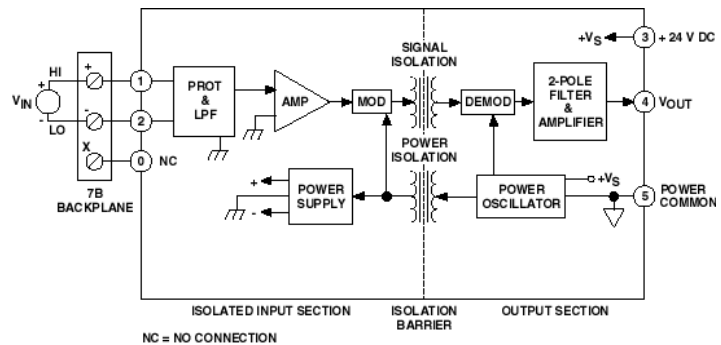
Figure 1. 7B30 Functional Block Diagram
