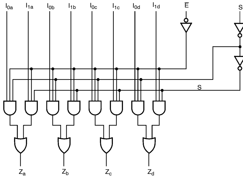
Figure 3. Logic Diagram
