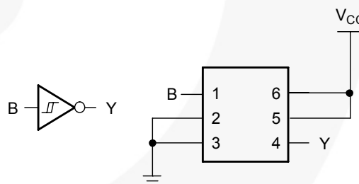
Figure 7. Inverter
