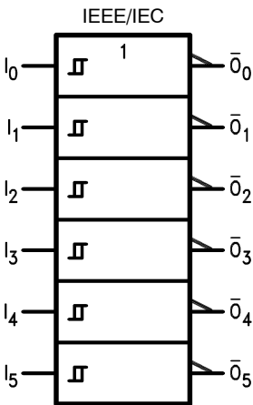
Figure 2. Logic Symbol
