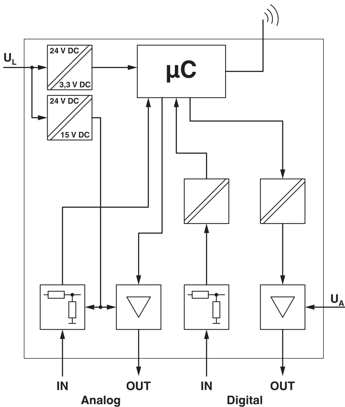
Block diagram
