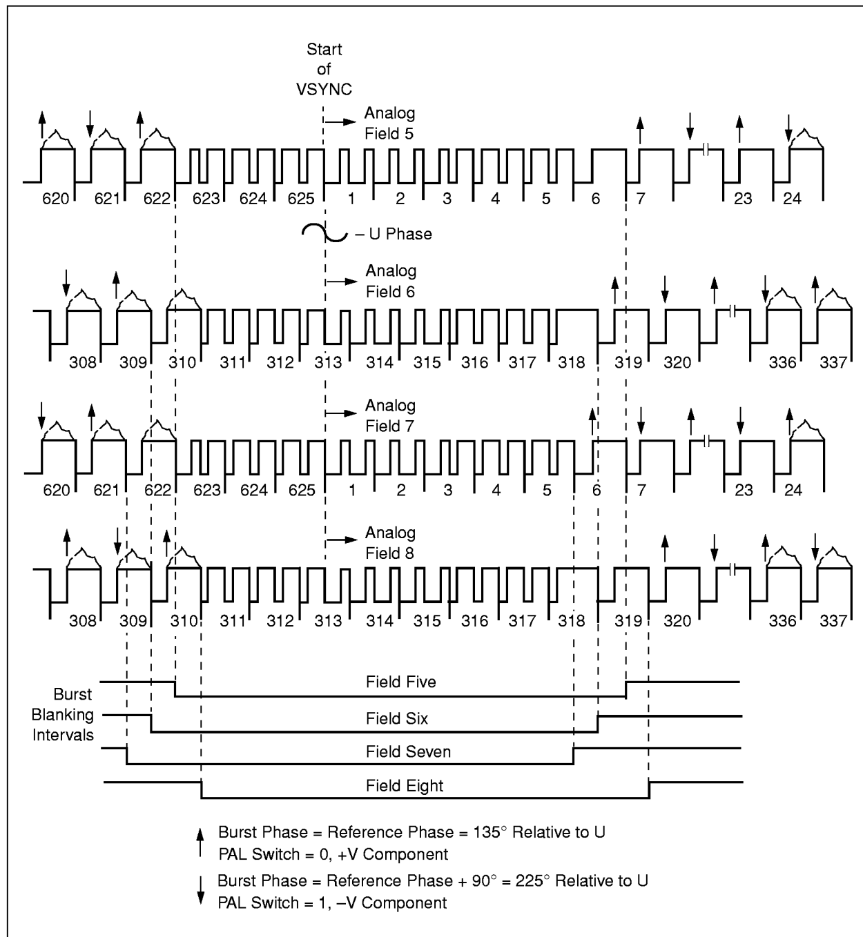
Figure 1-12. Interlaced 625-Line (PAL- \beta , D, G, H, I, N, N c ) Video Timing (Field 5–8)
