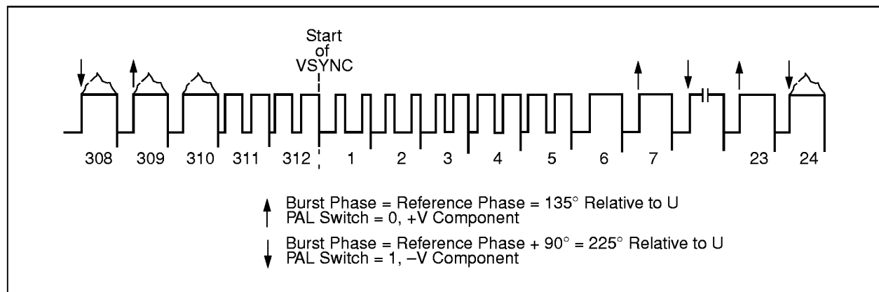
Figure 1-10. Noninterlaced 312-Line (PAL- \beta , D, G, H, I, N, N_c ) Video Timing ( EV\beta I = 0 )
