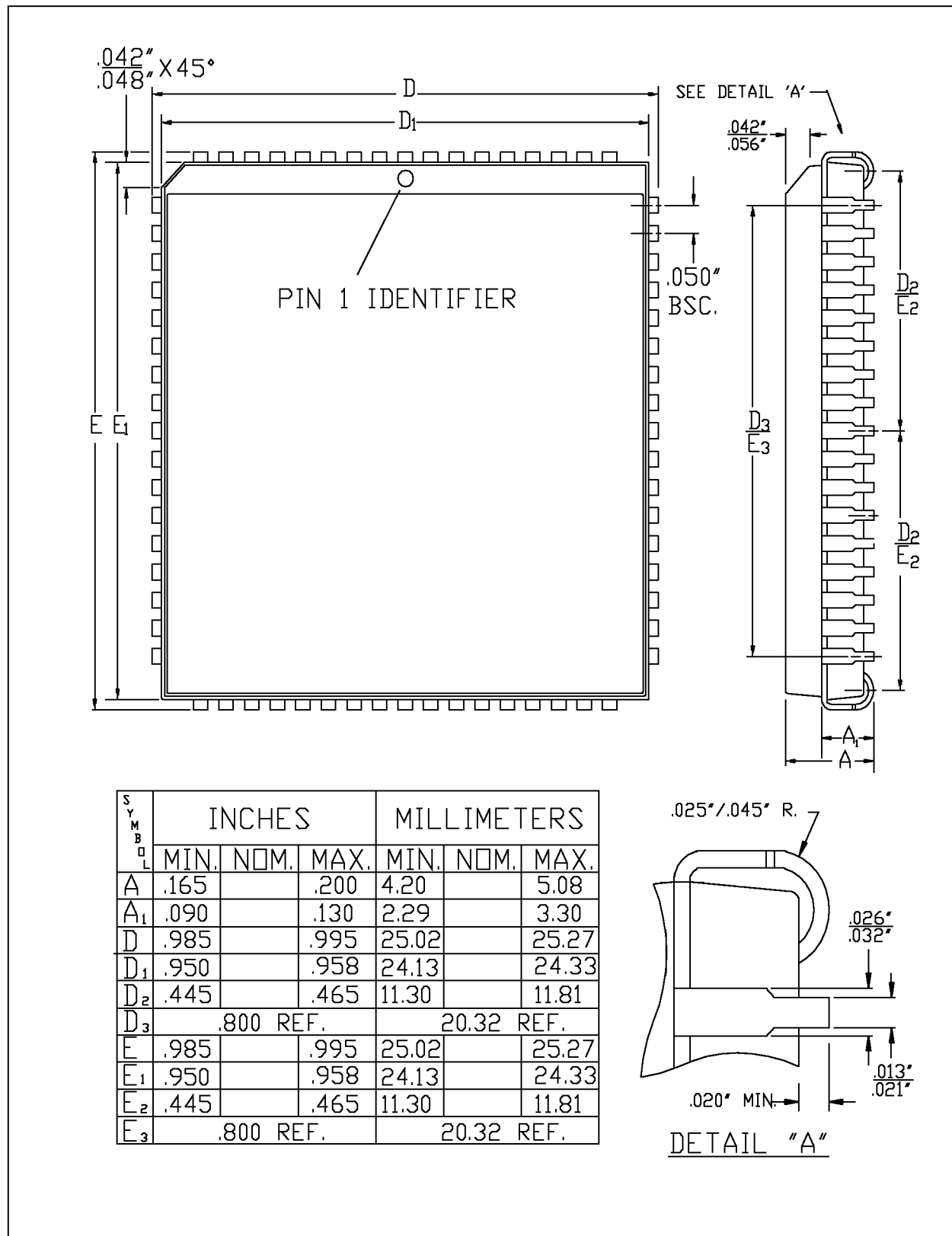
Figure 4-3. 68-Pin Plastic Leaded Chip Carrier (PLCC)
