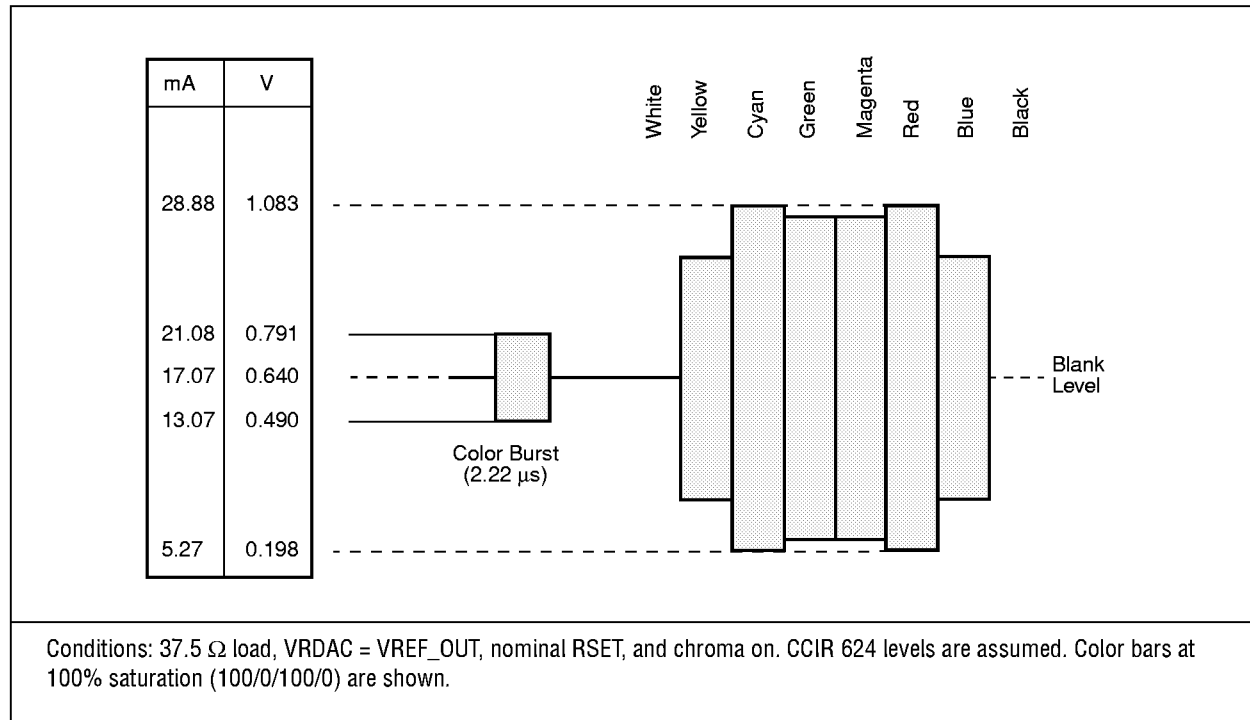
Figure 1-18. 625-Line (PAL- \beta , D, G, H, I, N, N c ) C (Chrominance) Video Output Waveform
