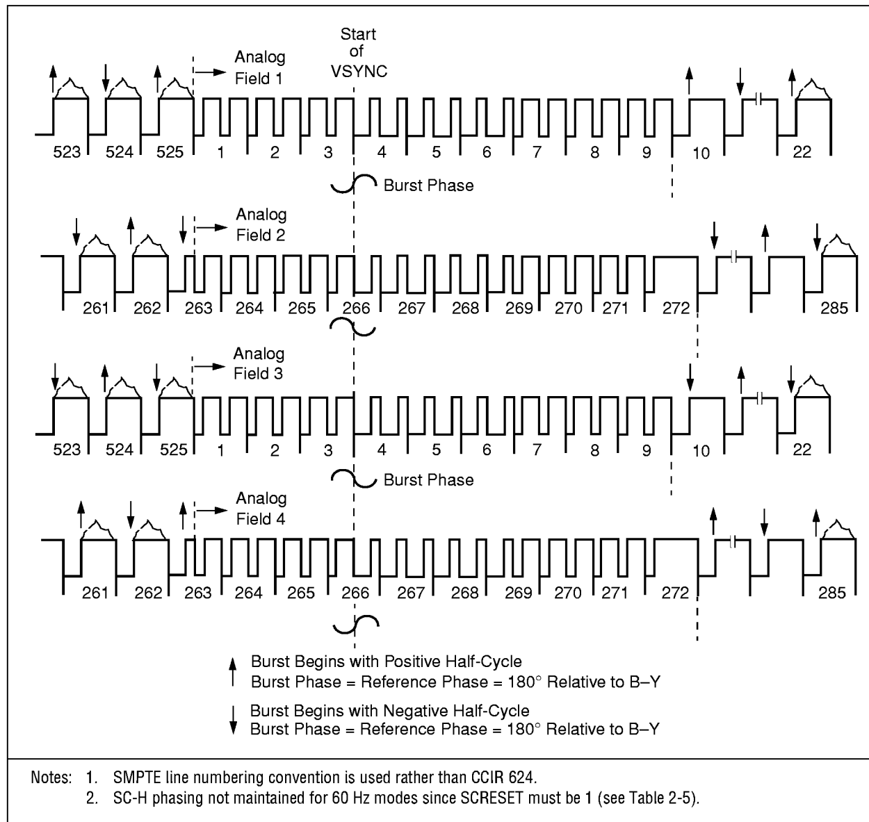
Figure 1-7. Interlaced 525-Line (NTSC) Video Timing (EVPI = 0)
