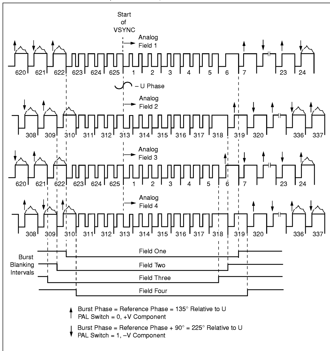
Figure 1-11. Interlaced 625-Line (PAL- \beta , D, G, H, I, N, N c ) Video Timing (Field 1-4)
