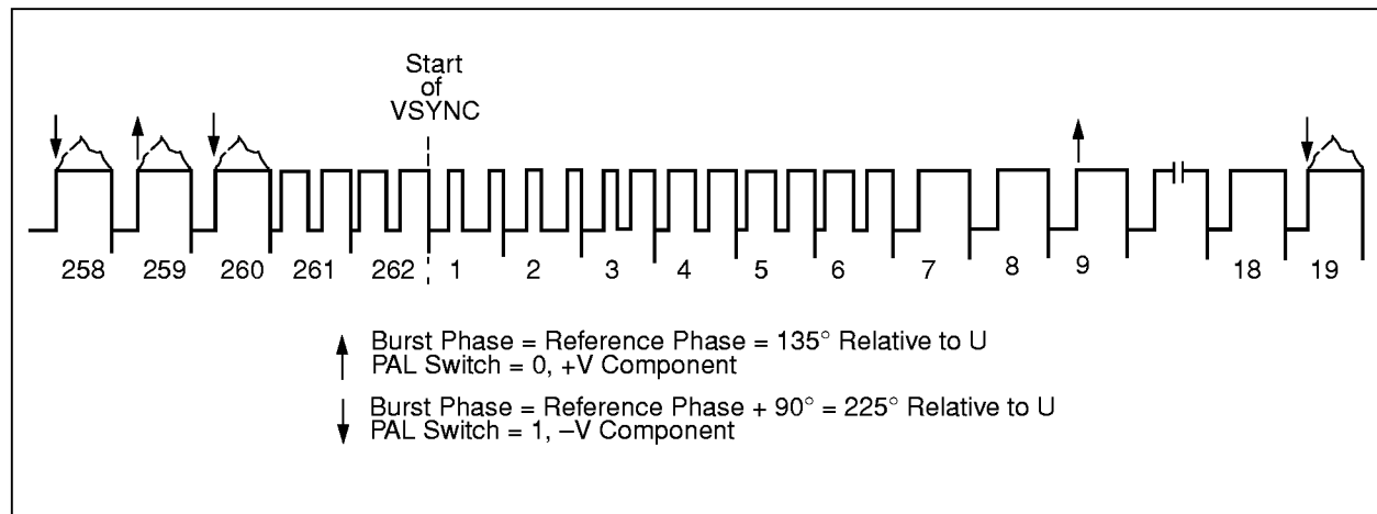
Figure 1-9. Noninterlaced 262-Line (PAL-M) Video Timing ( EV\beta I = 0 )
