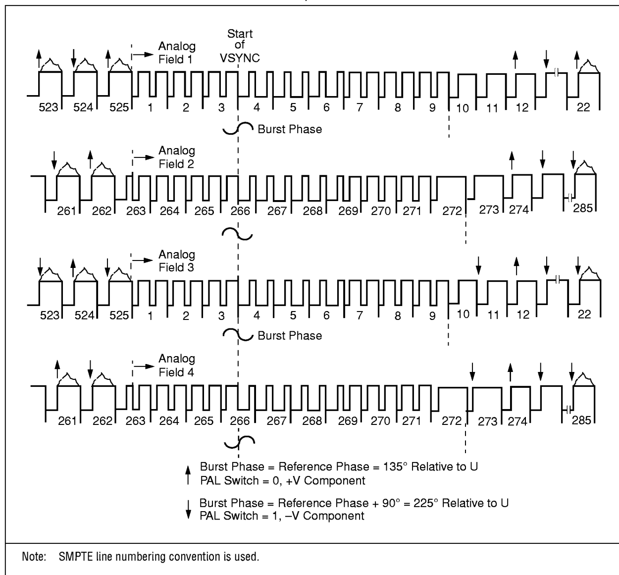
Figure 1-8. Interlaced 525-Line (PAL-M) Video Timing (EVBI = 0)
