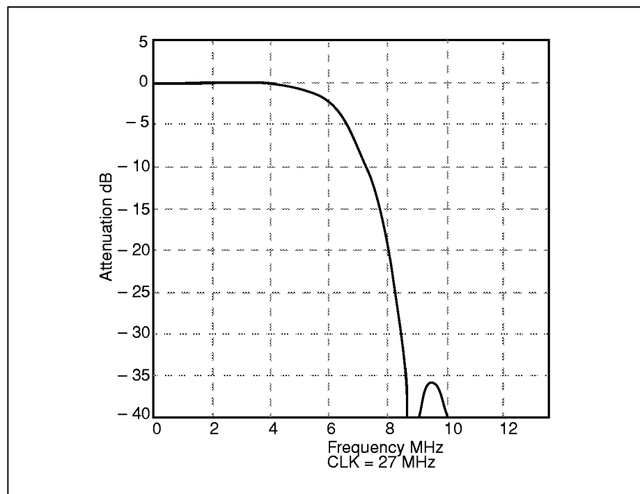
Figure 1-14. Internal 2x Upsampling Filter Response
