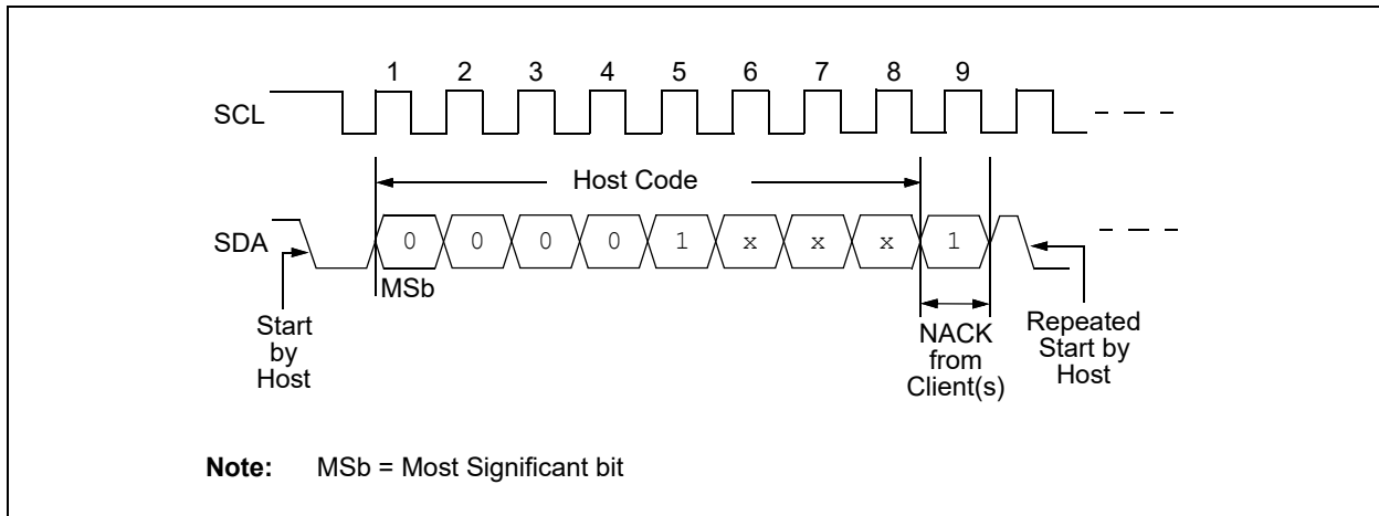
FIGURE 8-1: HIGH-SPEED MODE ENTRY SEQUENCE
