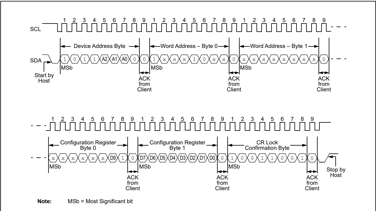
FIGURE 9-3: CONFIGURATION REGISTER LOCK SEQUENCE
