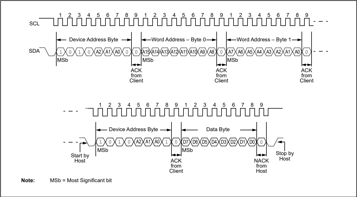
FIGURE 7-2: RANDOM READ
