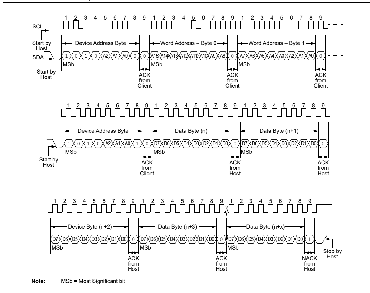
FIGURE 7-3: SEQUENTIAL READ
