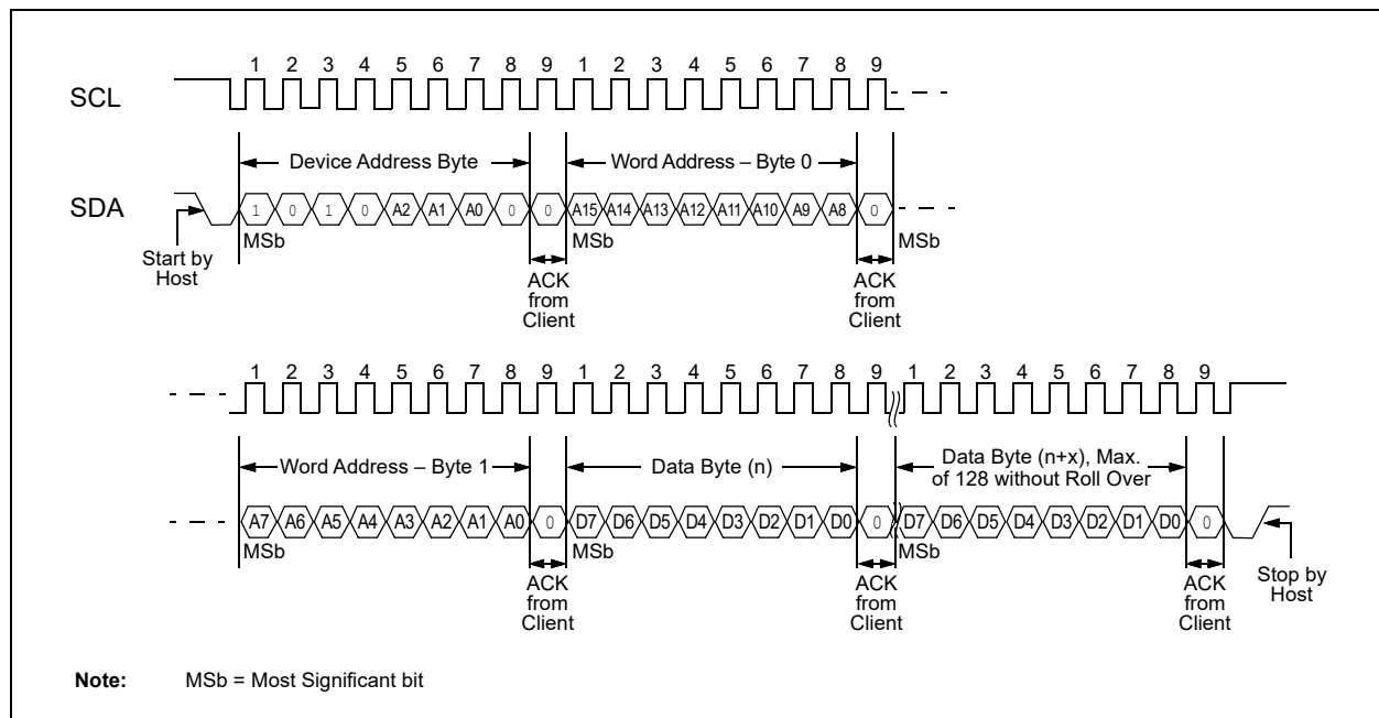
FIGURE 6-2: PAGE WRITE
