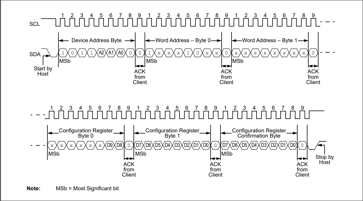
FIGURE 9-1: CONFIGURATION REGISTER WRITE SEQUENCE
